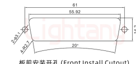
板前安装开孔 (Front Install Cutout)
