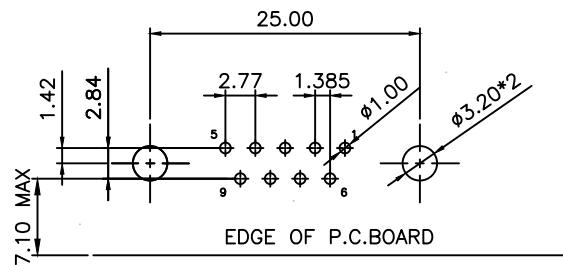
RECOMMENDED P.C.B LAYOUT (TOP VIEW) TOLERANCES: ±0.10mm
