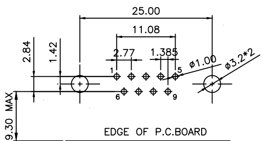
RECOMMENDED P.C.B LAYOUT (TOP VIEW) TOLERANCES: ±0.10mm
