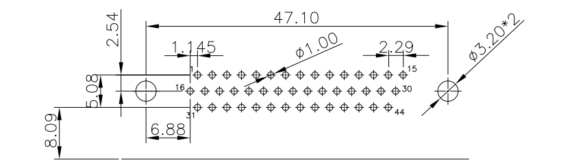
RECOMMENDED P.C.B LAYOUT (TOP VIEW) TOLERANCES: ±0.10mm
