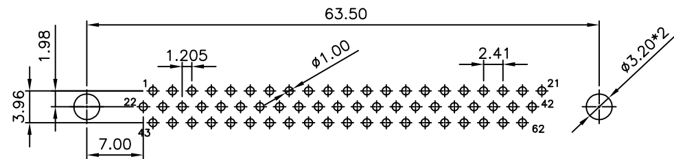
RECOMMENDED P.C.B LAYOUT (TOP VIEW) TOLERANCES: \pm 0.10\text{mm}
